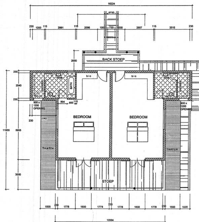
MAIN HOUSE 2 FIRST FLOOR PLAN
