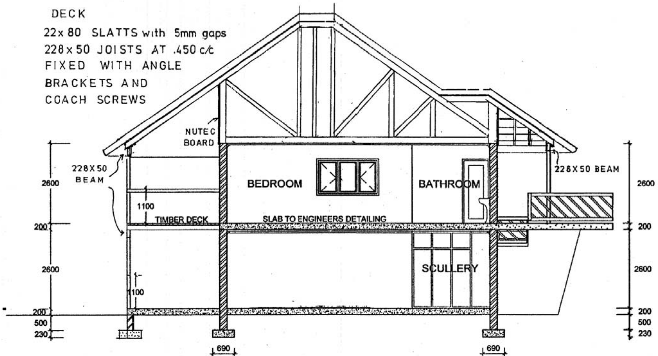
MAIN HOUSE 1 SECTION A-A
