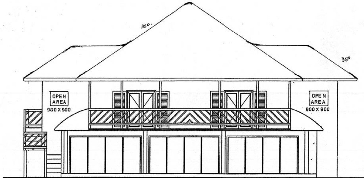
MAIN HOUSE 1 FRONT ELEVATION
