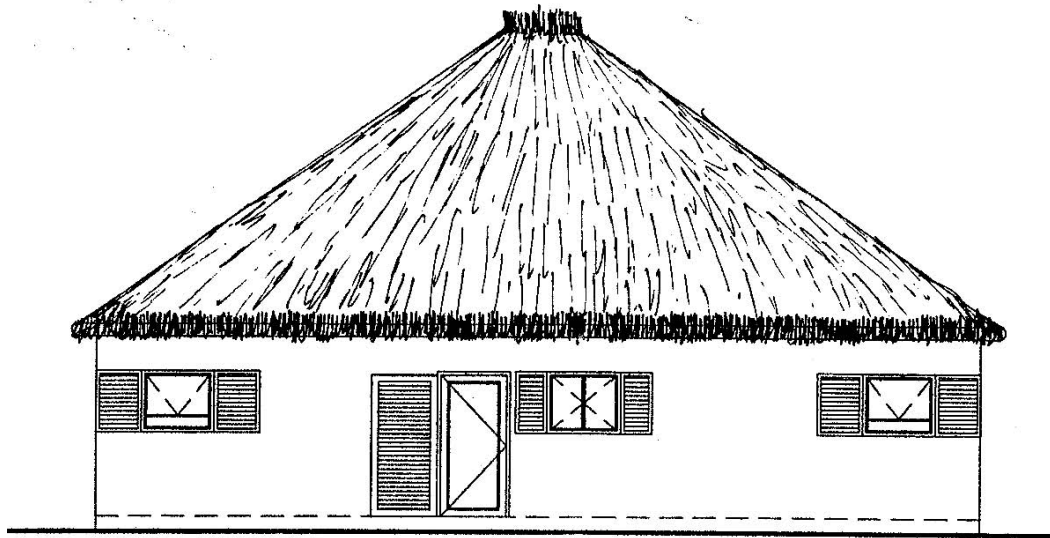
MANAGERS HOUSE BACK ELEVATION
