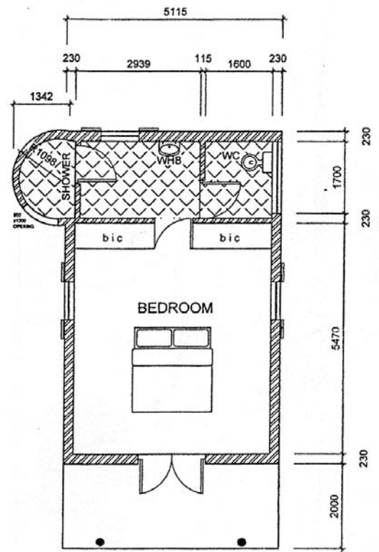
BEDROOM UNITS FLOOR PLAN
