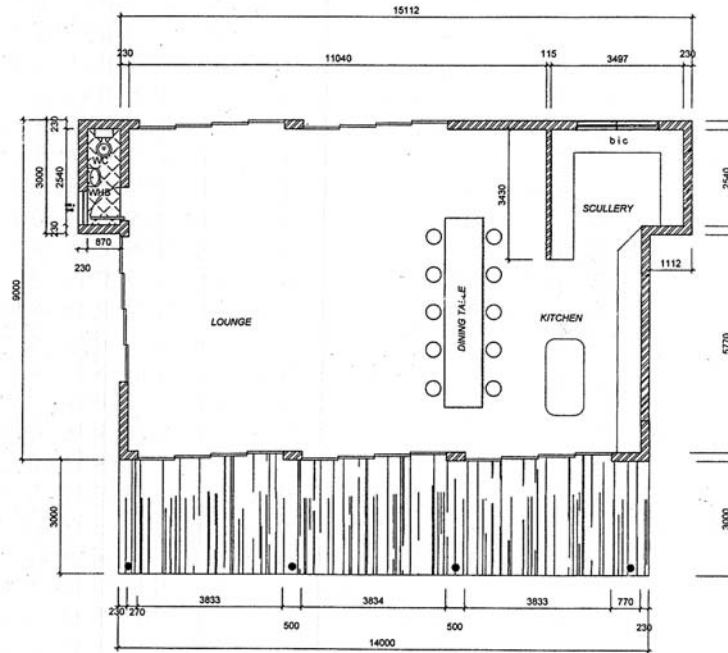
MAIN HOUSE 2 GROUND FLOOR PLAN
